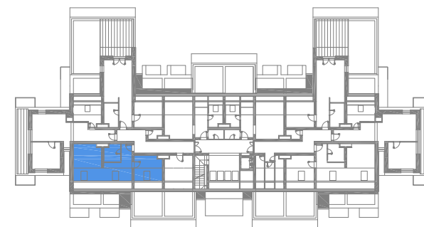
schéma pôdorysu 4. NP / scheme of the fourth floor
